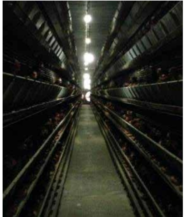
Figure 18. The LED lights installed in this house are too directional, too far apart and not bright enough. The combination of these factors leads to the obvious shadows on the floor and poor light uniformity along the cages.
